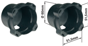
ACG8051 PAIR OF PLASTIC CONTAINERS to embed for FIT SYNCRO ACG8026
