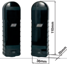
ACG8032 FIT SLIM* wall mounted range 20 m IP54 - 12/24V ac/dc
