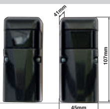
ACG8009 FIT METAL anti-vandals - wall mounted range 15 m IP55 - 12/24V ac/dc
